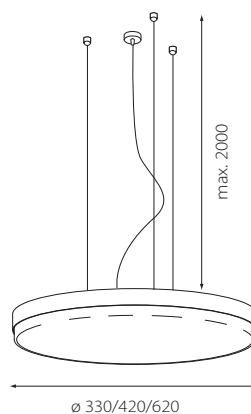
ø 330/420/620
