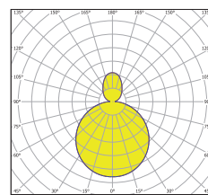
direct/indirect low output surface mounted
