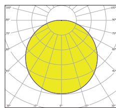
direct surface mounted/pendant
