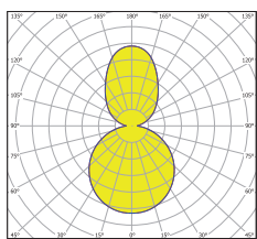
direct/indirect low output pendant
