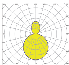
direct/indirect high output pendant
