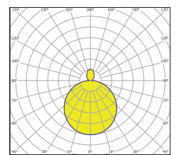
direct/indirect high output surface mounted
