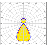
direct/indirect Reflector silver
