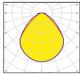
microprism direct
