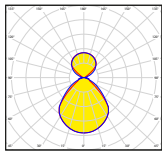
microprism direct/indirect
